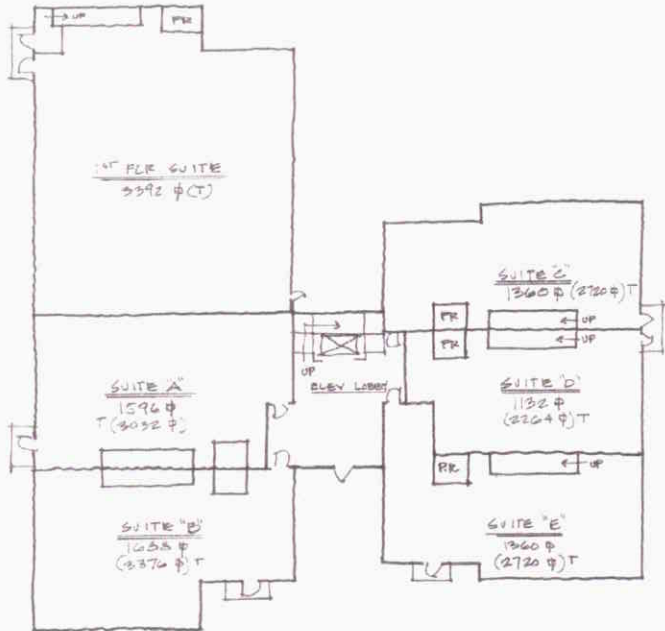
OFFICE BUILDING FIRST FLOOR PLAN
